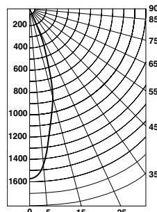
Candlepower Distribution (Candelas)
